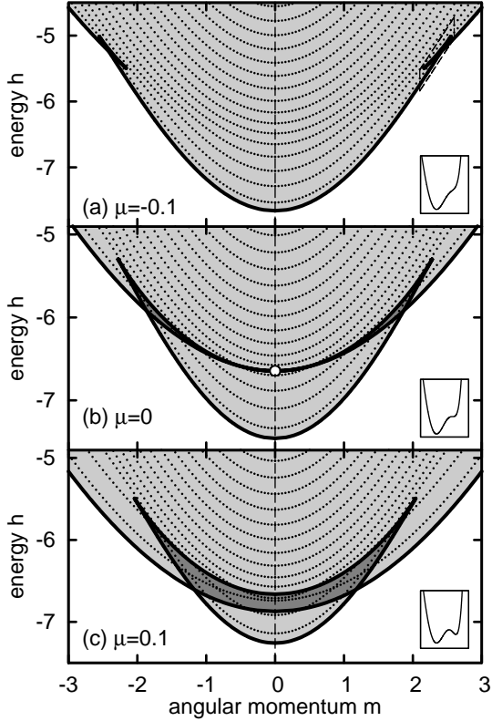
FIG. 13: Images of the energy-momentum map obtained from the octic potential V_{\text{oct}} [Eq. (13)] for \rho_1 = 1.5 and \rho_2 = 1.0 . The joint spectrum of commuting observables is represented by small dots and is determined with the Planck constant set to \hbar = 0.05 . The insets show the octic potential V_{\text{oct}} . (a) Control parameter \mu = -0.1 . The dashed curves delimit the area that is enlarged in Fig. 14. (b) Control parameter \mu = 0 . (c) Control parameter \mu = 0.1 .
