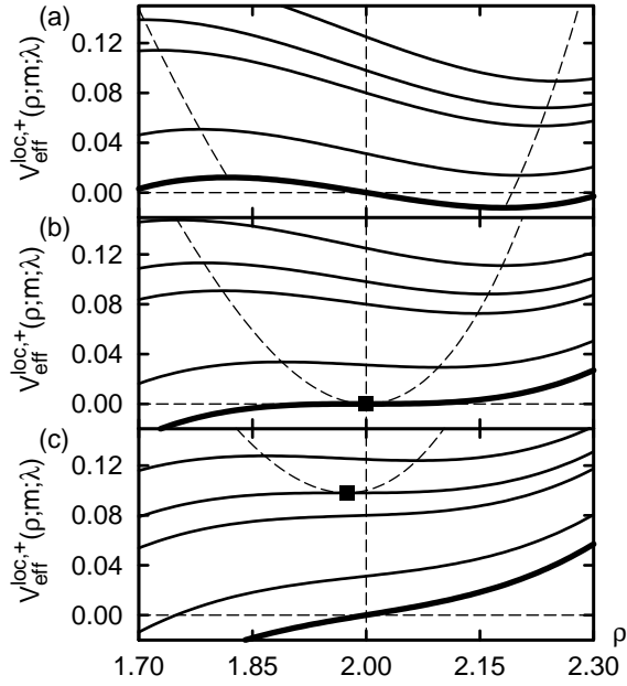
FIG. 8: Local effective potential V_{\text{eff}}^{\text{loc,+}}(\rho; m; \lambda) for \rho_0 = 2 and a fixed set of five values of angular momentum m . The effective potential with m = 0 is represented by a thick curve. Angular momentum increases (values: m_1 = 0.5, m_2 = 0.8, m_{\text{deg,II}}(0.1) \simeq 0.886, m_3 = 1.0 ) when jumping from one potential curve to the upper one. Filled squares indicate degenerate critical points. Positions of the minima and maxima of the effective potentials are indicated by the dashed curves. (a) Control parameter \lambda = -0.1 . (b) Control parameter \lambda = 0 . (c) Control parameter \lambda = 0.1 .
