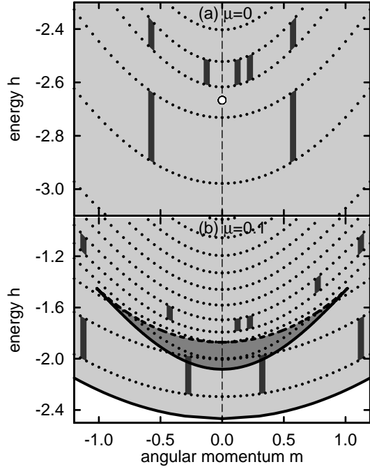
FIG. 12: (a) Enlargement of Fig. 11(b) in the vicinity of the singularity. (b) Enlargement of the two sheets seen on Fig. 11(c).
