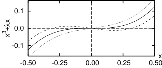
FIG. 3: Fold catastrophe: the germ ( \lambda = 0 , solid curve) and its unfolding for \lambda = -0.1 (dashed line) and \lambda = 0.1 (dotted line).
