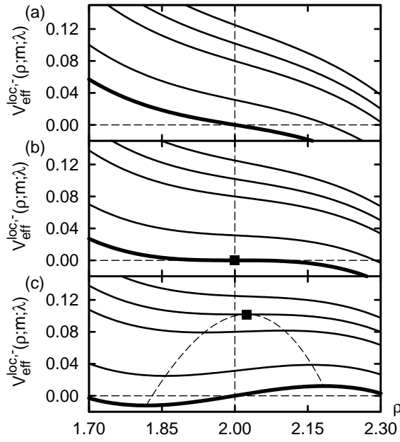
FIG. 4: Local effective potential V_{\text{eff}}^{\text{loc},-}(\rho; m; \lambda) for \rho_0 = 2 and a fixed set of five values of angular momentum m . The effective potential with m = 0 is represented by a thick curve. Angular momentum increases (values: m_1 = 0.5, m_2 = 0.8, m_{\text{deg},1}(0.1) \simeq 0.903, m_3 = 1.0 ) when jumping from one potential curve to the upper one. Filled squares indicate degenerate critical points. (a) Control parameter \lambda = -0.1 . (b) Control parameter \lambda = 0 . (c) Control parameter \lambda = 0.1 . Positions of the minima and maxima of the effective potentials are indicated by the dashed curves.
