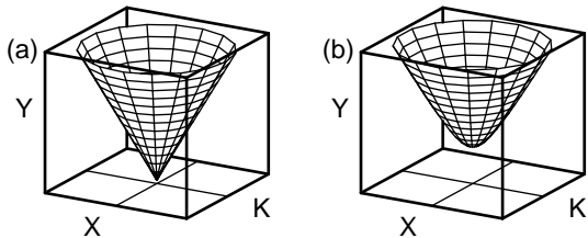
FIG. 2: Reduced phase spaces of a two degrees of freedom SO(2) invariant Hamiltonian in the space of invariant polynomials (X, K, Y) . (a) Singular reduced phase space for m = 0 . (b) Smooth reduced phase space for m = 2 .
