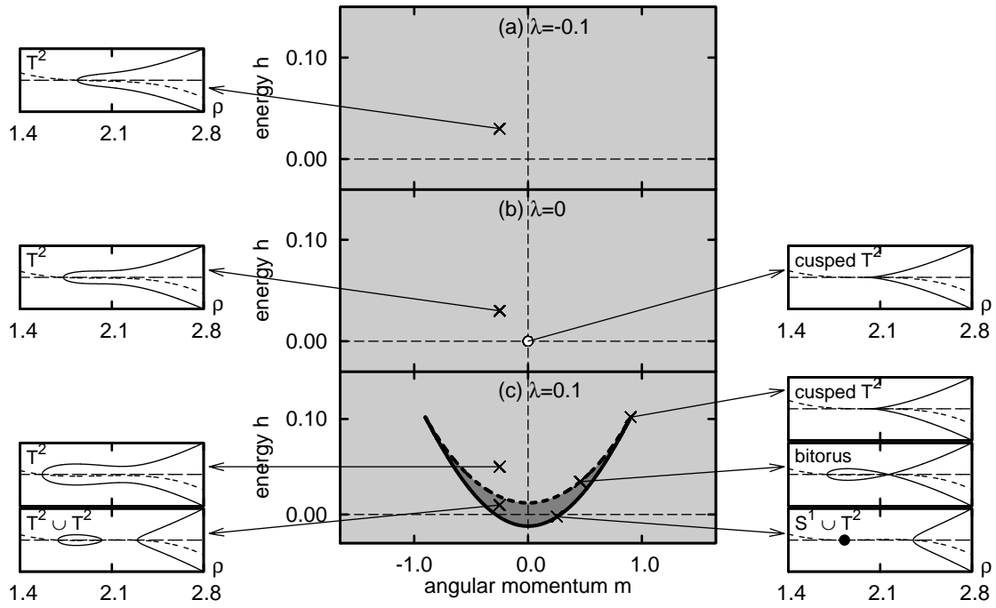
FIG. 7: Images of the energy-momentum map in case I. The preimage of a point in the light grey areas is one torus while the preimage of a point in the dark grey area consists of two tori. Selected points in the image of the energy-momentum map are marked by a cross and the figures attached to them show the effective potential (dashed curve), the energy (horizontal dashed curve), and the conjugate momenta p_\rho (solid curve). (a) Control parameter \lambda = -0.1 . (b) Control parameter \lambda = 0 . (c) Control parameter \lambda = 0.1 .
