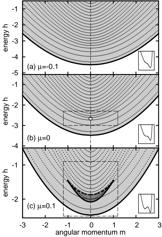
FIG. 11: Images of the energy-momentum map obtained from the octic potential V_{\text{oct}} [Eq. (13)] for \rho_1 = 1.0 and \rho_2 = 1.5 . The joint spectrum of commuting observables is represented by small dots and is determined with the Planck constant set to \hbar = 0.05 . The insets show the octic potential V_{\text{oct}} . (a) Control parameter \mu = -0.1 . (b) Control parameter \mu = 0 . The dashed rectangle delimits the area that is enlarged in Fig. 12(a). (c) Control parameter \mu = 0.1 . The dashed rectangle delimits the area that is enlarged in Fig. 12(b).
