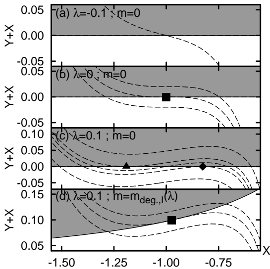
FIG. 6: Projections of the reduced phase spaces (grey domains) and energy level sets (dashed curves) in the (X, Y+X) space of invariant polynomials for the case I with \rho_0 = 2 . The symbols of Fig. 5 are used to label the singular intersection points.
