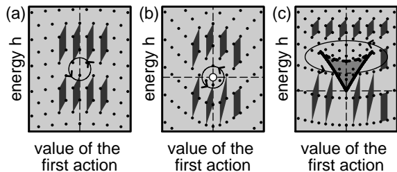
FIG. 1: Typical open subsets of the image of the energy-momentum map for a two degrees of freedom completely integrable system when the first action is a global action. The lattice of dots represents the joint spectrum of commuting observables and the filled quadrilaterals describe the evolution of an elementary cell along one closed loop. (a) Open subset with only regular values. (b) Open subset with regular values and one singular value indicated by the circle. (c) Open subset with two sheets of regular values glued along a singular dashed curve.
