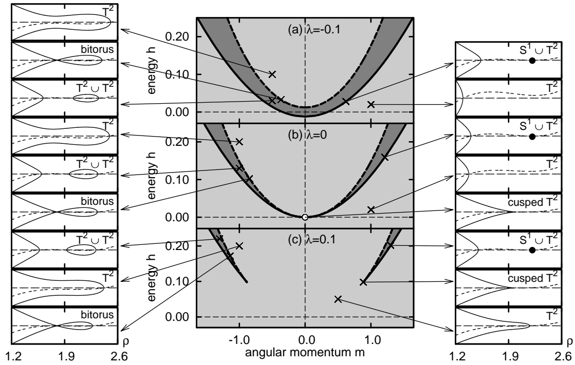
FIG. 10: Images of the energy-momentum map in case II. The preimage of a point in the light grey areas is one torus while the preimage of a point in the dark grey areas consists of two tori. Selected points in the image of the energy-momentum map are marked by a cross and the figures attached to them show the effective potential (dashed curve), the energy (horizontal dashed curve), and the conjugate momenta p_\rho (solid curve). (a) Control parameter \lambda = -0.1 . (b) Control parameter \lambda = 0 . (c) Control parameter \lambda = 0.1 .
