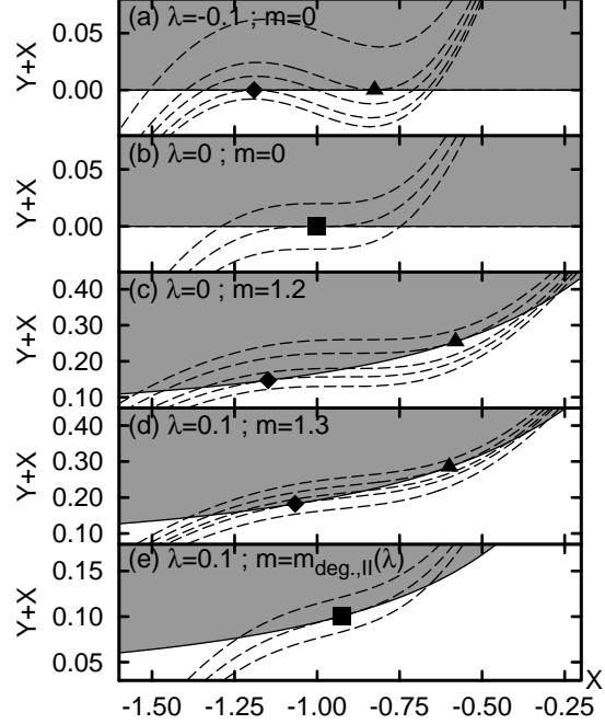
FIG. 9: Projections of the reduced phase spaces (grey domains) and energy level sets (dashed curves) in the (X, Y + X) space of invariant polynomials for the case II with \rho_0 = 2 . The symbols of Fig. 5 are used to label the singular intersection points.
