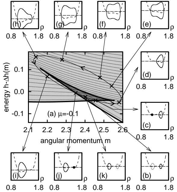
FIG. 14: (a) Enlargement of Fig. 13(a). The quantum eigenstates have been determined with the Planck constant \hbar = 0.005 . The energy axis is shifted by a linear function \Delta h of the angular momentum m : \Delta h(m) = 1.6m - 9.06 . (b-k) Effective potential (dashed curve), energy (horizontal dashed line) and radial momentum \pm p_\rho(\rho) (solid curves) are drawn for ten representative points in the image of the energy-momentum map. The small filled circles represent \pm p_\rho(\rho) curves reduced to one point. The evolution of a torus from panel (b) to panel (k) is seen in the continuous curves. Panels (b) and (k) have two regular tori: one is drawn as a continuous curve and the other one is drawn as a dotted curve.
